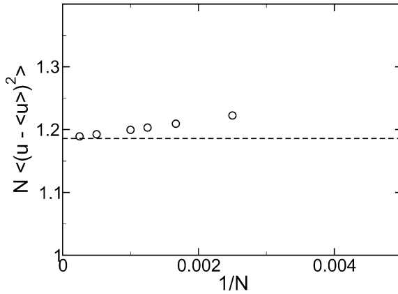
Fig. 4. The O(1/N) shift in the variance of the surface magnetization is shown (circles). Also shown is the prediction from Eq. (84) (dashed line). We use f(m) = km^2/2 + 1 and d(m) = 0 with k/\mu = 2 and \mu = 5 .
